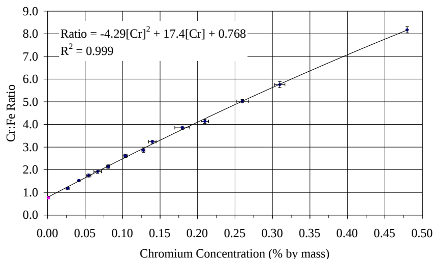
Calibration curve for chromium in mild-steel using a 30 m fibre-optic probe LIBS instrument
